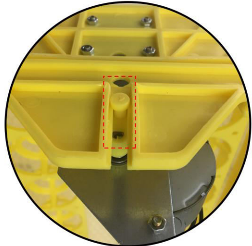
4、 Ensure egg tray matched motor shaft connector (48&56 eggs incubator)
